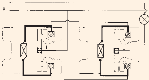
Changeover switch with pilot lamp
