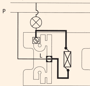
Single pole switch with pilot lamp
