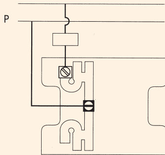
Changeover switch with pilot lamp
