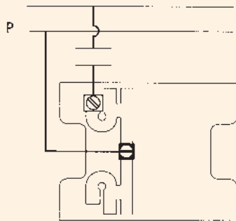
Changeover switch with pilot lamp
