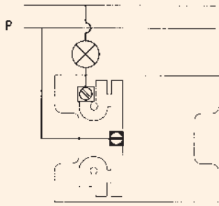
Single pole switch
