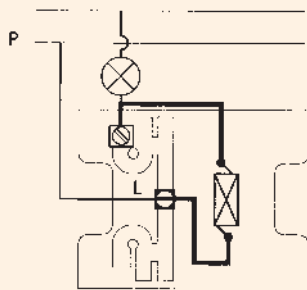
Single pole switch with pilot lamp
