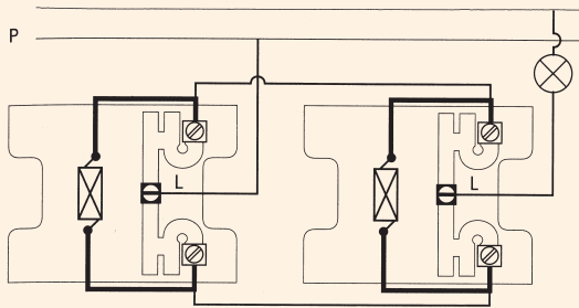
Changeover switch with pilot lamp
