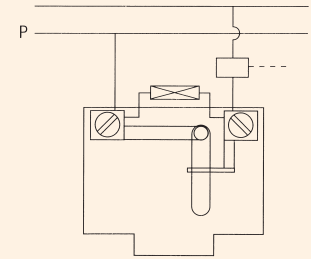
Push-button with pilot lamp
