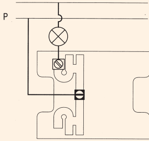
Single pole switch
