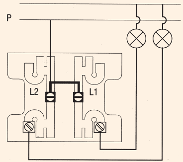
Push-button with pilot lamp
